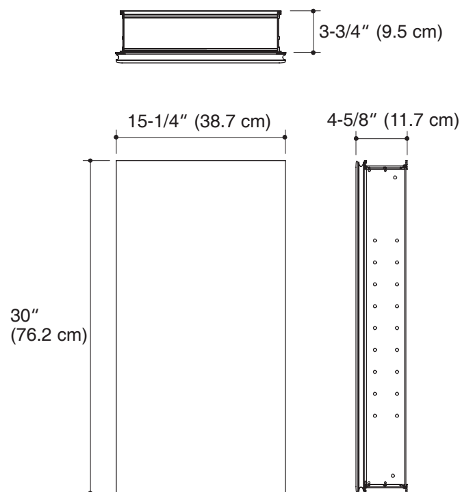
Product Diagram
