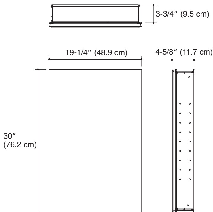
Product Diagram
