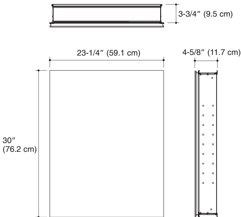
Product Diagram
